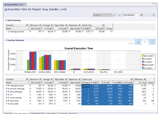
Figure 1 – Example of RapiTime's execution time report
