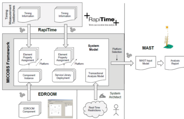
Figure 2: Toolchain integration
