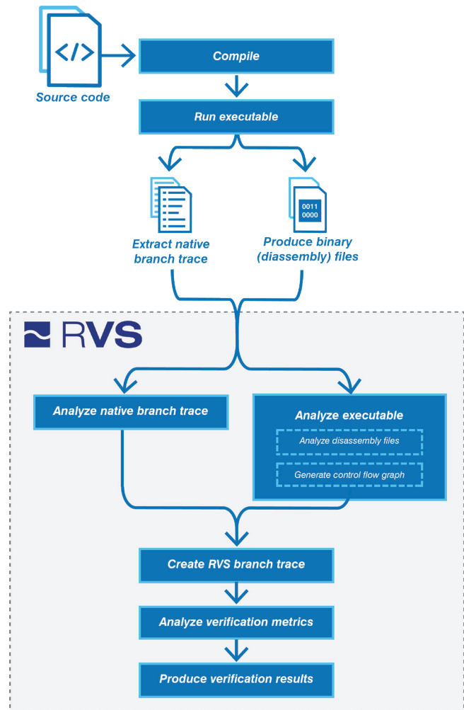
Figure 1. RapiTask Zero verification process
