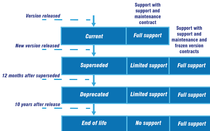
Figure 1. Rapita software product life cycle
